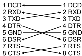
DB9 (EX-45034IS)
