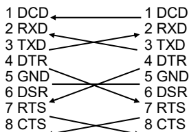
DB9 (EX-1344HMV)
