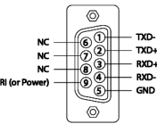
RS-422 and RS-485 4-wire Pin Assignment
